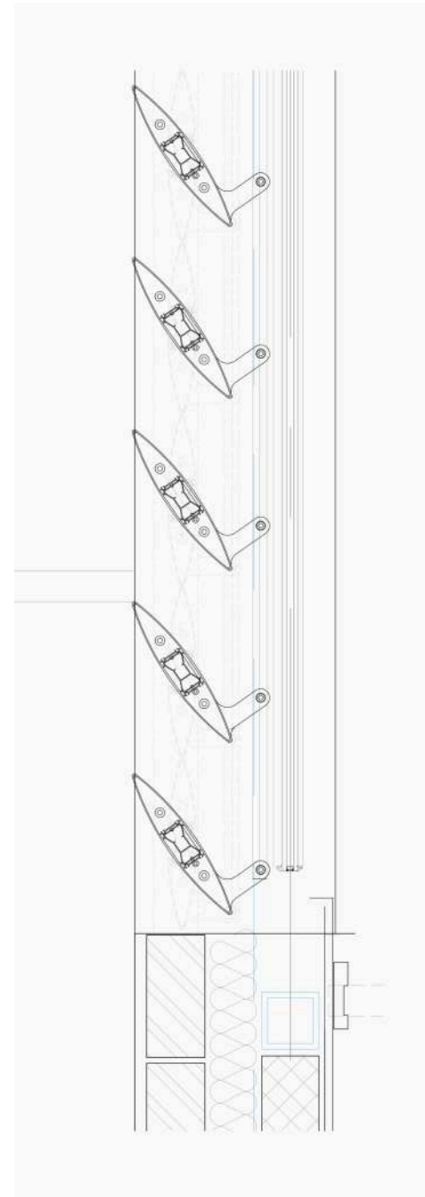
LOUVRE DETAIL PLAN
